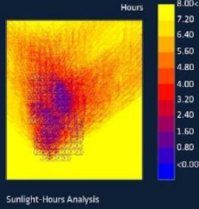
Sunlight-Hours Analysis
